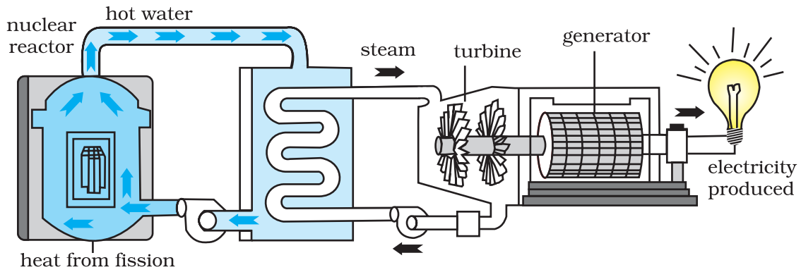
Fig. 3.19 : Nuclear Energy
